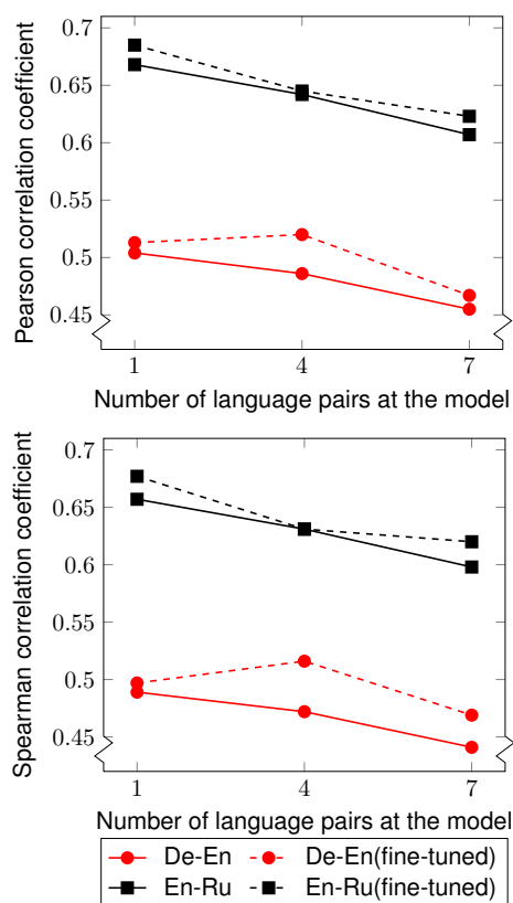
Figure 2: Pearson and Spearman correlation coefficients for LAME model and different number of language pairs in training dataset. We show average over three runs. Test dataset: newstest2016
