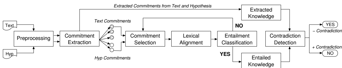
Figure 1: System Architecture.
