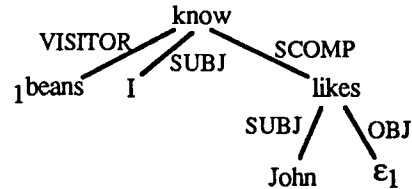
Figure 2. Dependency tree of the sentence "Beans I know John likes", given the grammar G_1 .
