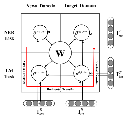
Figure 1: Overview of the proposed model.
