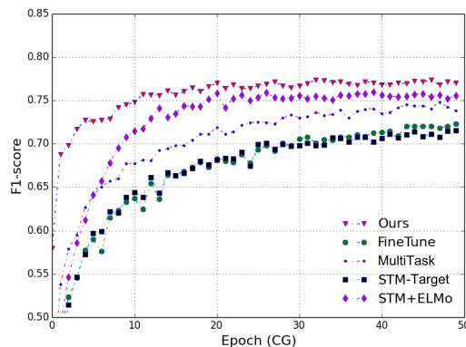
Figure 3: Development results on 13CG.
