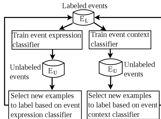
Figure 1: The Co-Training Model
