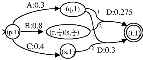
Figure 5: Determinized bottom-up tree-to-weight transducer
