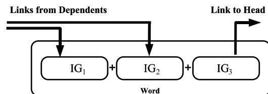
Figure 2: Dependency Links and IGs
