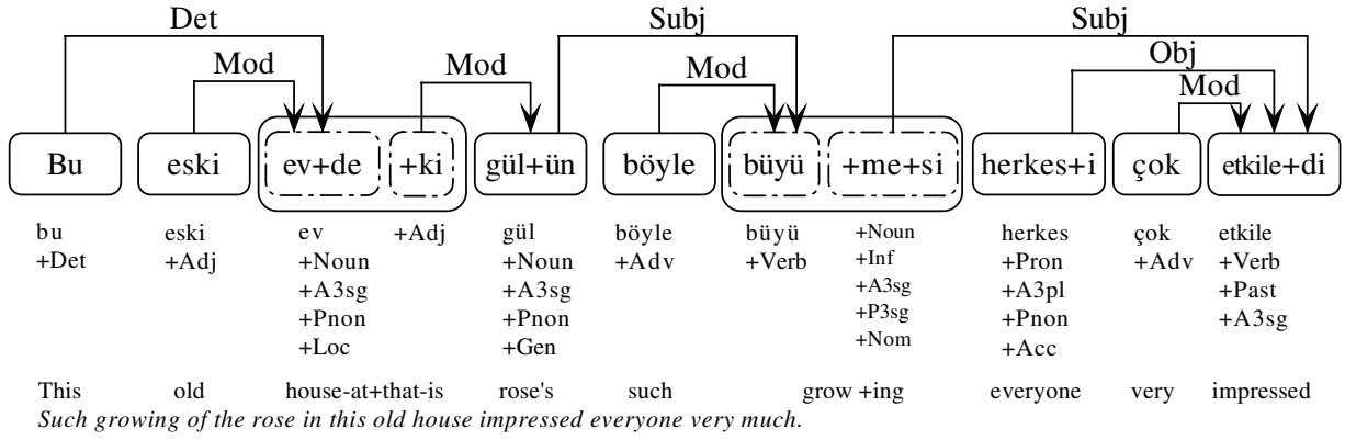
+’s indicate morpheme boundaries. The rounded rectangles show the words while the inflectional groups within the words that have more than 1 IG are emphasized with the dashed rounded rectangles. The inflectional features of each inflectional group as produced by the morphological analyzer are listed below.
