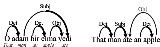
Figure 1: Dependency Relations for a Turkish and an English sentence
