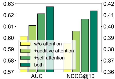
(b) Attention mechanisms of different kinds.
