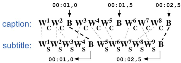
Figure 4: Example of Semantic-based projection.
