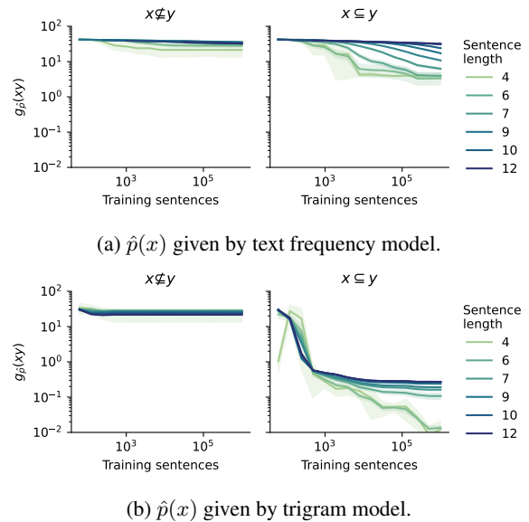
Figure 3: Plot of g_{\hat{p}}(x, y) = \log \frac{\hat{p}(xy)}{\hat{p}(x)\hat{p}(y)} - \log \frac{\hat{p}(yy)}{\hat{p}(y)\hat{p}(y)} as a function of the number of sentences in the training corpus and the length |xy| . Given the true distribution p , g_p(x, y) = 0 iff x entails y . We exclude pairs x, y where both xy and yy are absent from the training data.
