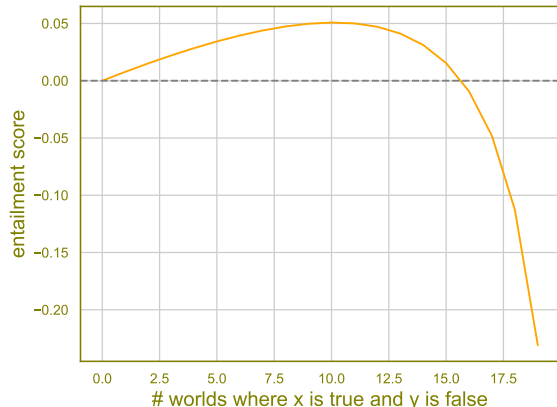
Figure 1: The entailment test score between x and y as a function of the number of worlds where x is true but y is false. Entailment (left intercept with 0) and near contradiction (right intercept with 0) look the same!
