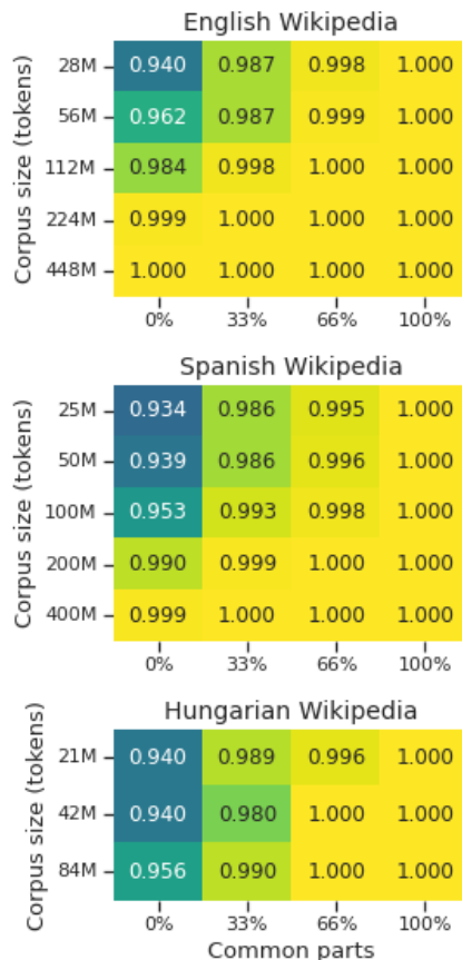
Figure 5: P@1 scores of RCSLS mappings of embeddings from Wikipedia parts of various overlap ratio and size.
