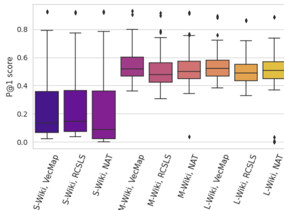
Figure 1: Distributions of BLI scores of embedding mappings using different methods and corpus types.
