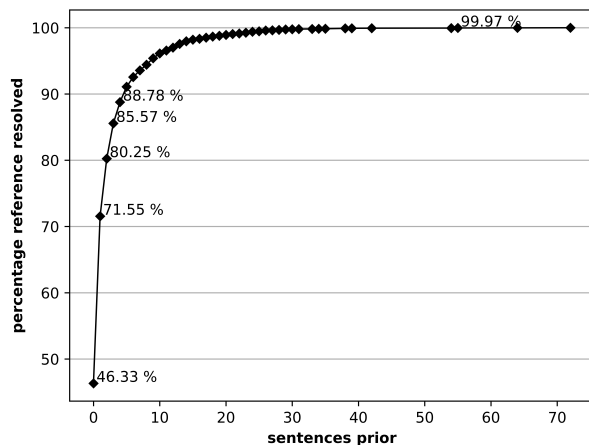
Figure 1: The likelihood that a reference can be found within the previous x sentences in the original context.
