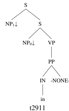
Figure 12: Elementary tree used in Sentence 7.
