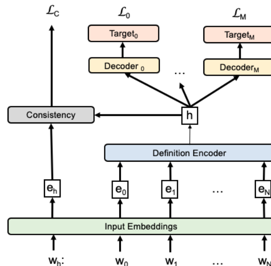
Figure 1: Model architecture for multi-task learning auto-encoder for embedding words from their structured dictionary entries. Input tokens are embedded using the Input Embeddings layer, and the n tokens in the definition of headword w_h are passed to the Definition Encoder to produce the definition embedding h . This embedding should be consistent (low distance) with the embedding of the definition headword e_h . M possible output tasks can be used, each with its own decoder which needs to reconstruct the Target.
