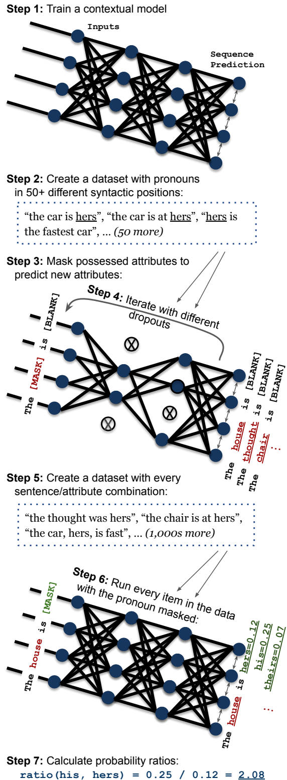
Figure 1: An overview of our workflow for bias-detection. We generate 1000s of unique sentences to test the bias, from an initial set of 50+ sentences created with maximally diverse contexts, utilizing masked models with dropouts to generate a list of candidate possessed attributes.
