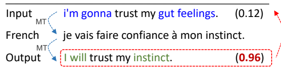
Figure 2: Formality discrimination for FST. The numbers following the sentences are formality scores predicted by a formality discriminator. The pair (connected by the red dashed arrow) that obtains significant formality improvement will be kept as augmented data.
