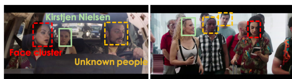
Figure 5: The two green bounding boxes are coreferential since they are both linked to “Kirstjen Nielsen”, and two red bounding boxes are coreferential based on face features. The yellow bounding boxes are unlinkable and also not coreferential to other bounding boxes.
