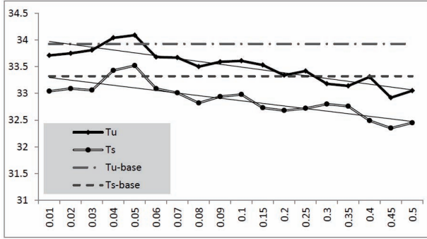
Figure 1: Results (BLEU) of evaluating the SMT systems for Dev. ( T_u ) and test sets ( T_s ). The X-axis shows the percentage of sentence pairs removed from the training corpus. The baseline scores are illustrated by T_u -base and T_s -base
