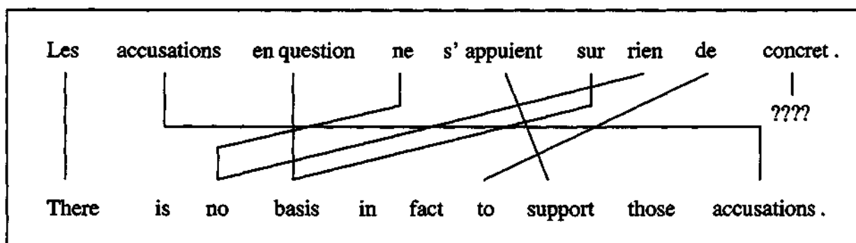
Figure 1: An example of TM-Align Output
