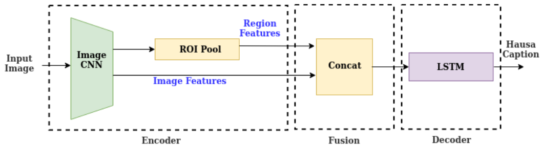
Figure 3: Architecture of the region-specific image caption generator.
