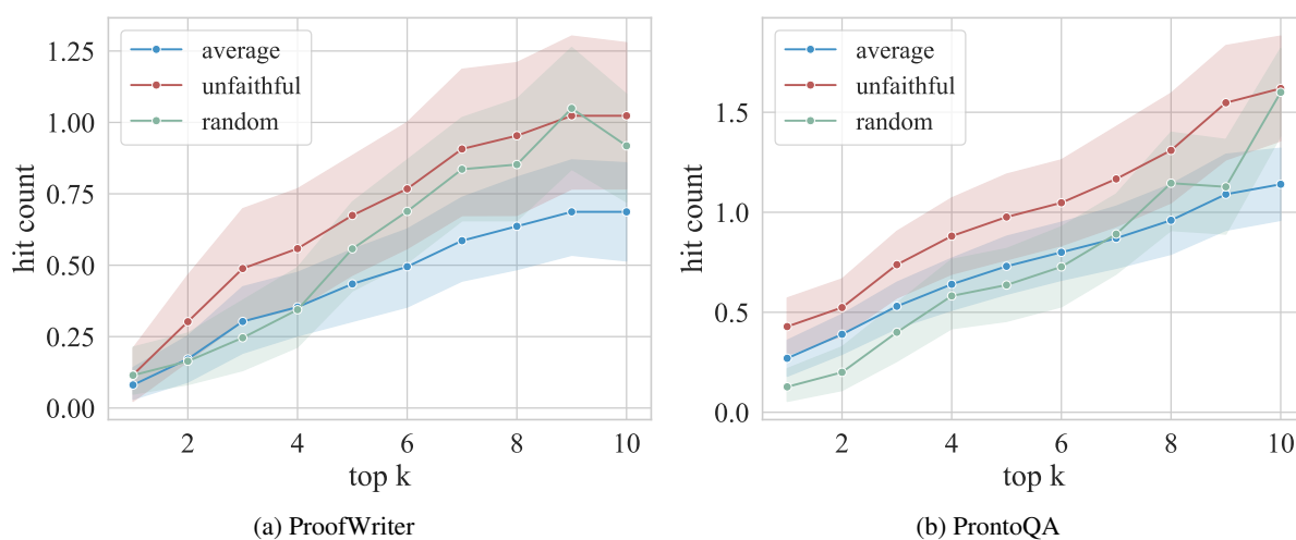
Figure 20: Comparison of correct statements recall counts (Llama2-13B).
