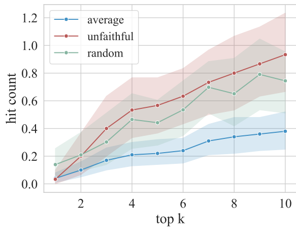
(a) ProofWriter
