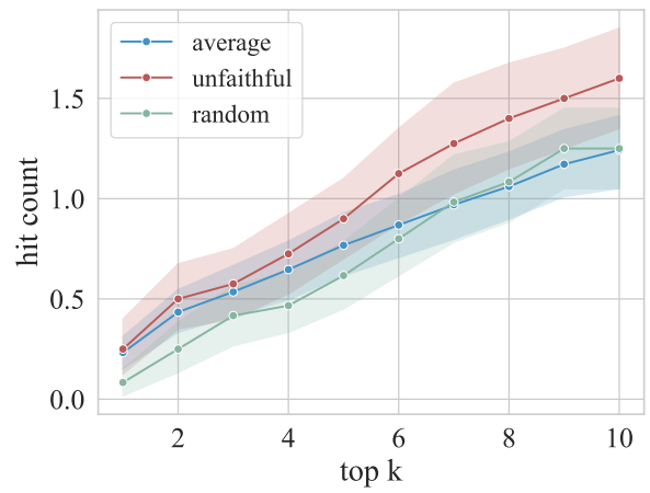
(b) ProntoQA
