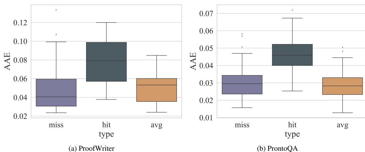
Figure 19: Comparison of information interaction between contexts and CoTs under three settings (Mistral-7B).
