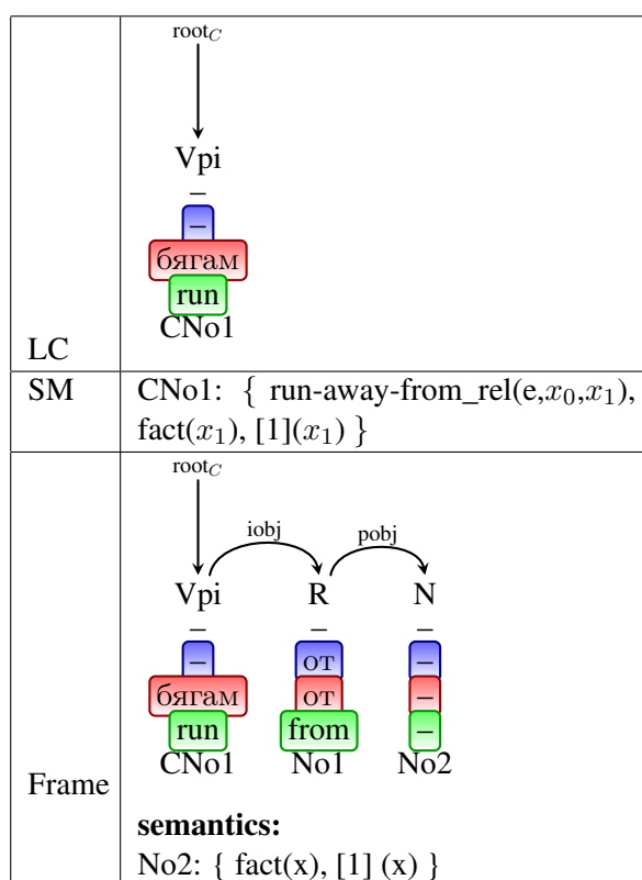
Figure 6: Lexical entry for the verb бягам "byagam", ‘run’).
