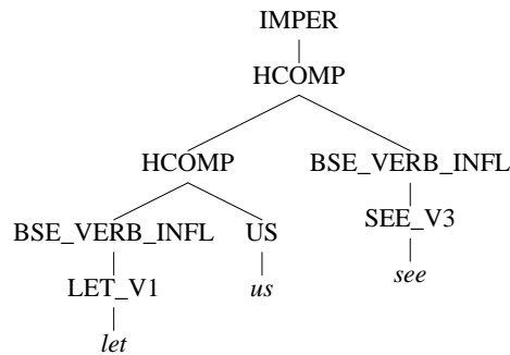
Figure 1: Derivation tree for the sentence Let us see
