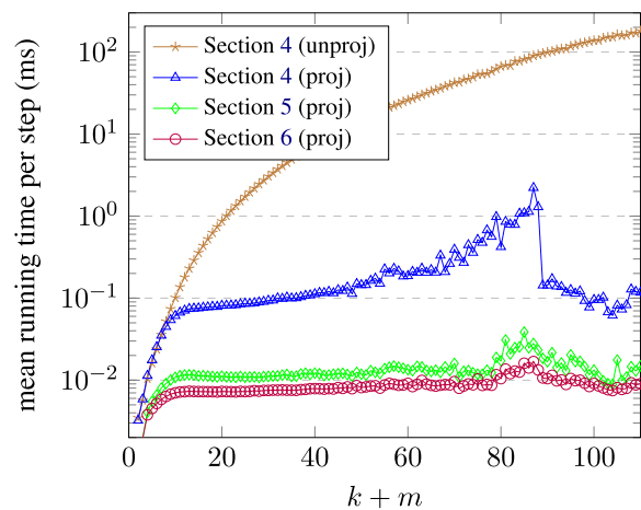
Figure 9: Mean running time per step (milliseconds) against length of input, for projectivized and unprojectivized trees.
