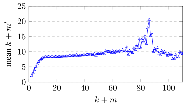
Figure 10: Mean k + m' against k + m .
