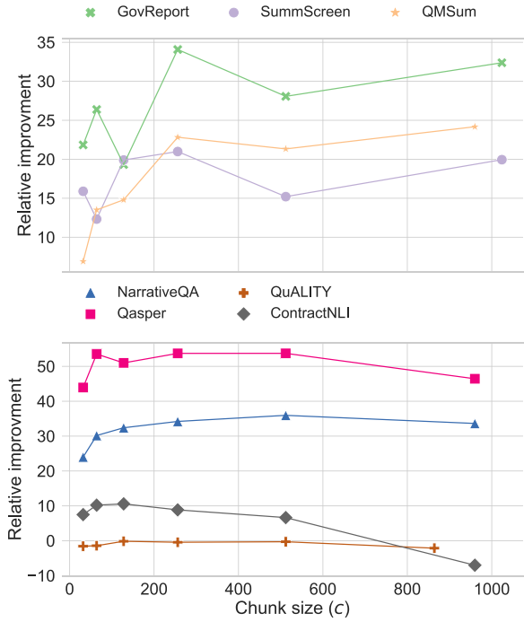
Figure 5: \text{BART}_{\text{base}} -SLED relative improvement compared to \text{BART}_{\text{base}} results, when varying the SLED’s chunk size (i.e., c ), fixing the maximum input length to 16K. Top: Summarization datasets. The y -axis measures relative improvement of Rouge-2. Bottom: QA and NLI datasets. The y -axis measures relative improvement of exact match for QuALITY and ContractNLI and F_1 for NarrativeQA and Qasper.
