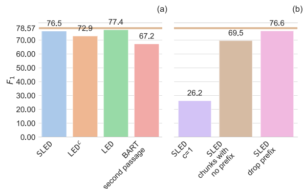
Figure 4: F_1 results on our HotpotQA’s development set (Yang et al., 2018). (a) SLED reaches an F_1 that is close to the oracle \text{BART}_{\text{base}} (horizontal line), outperforming a model with access to the paragraph that contains the answer (“second paragraph”). This shows that SLED effectively fuses information from two chunks. See text for further explanation on each model. (b) Ablations on SLED’s architecture, see §4.3 for details.
