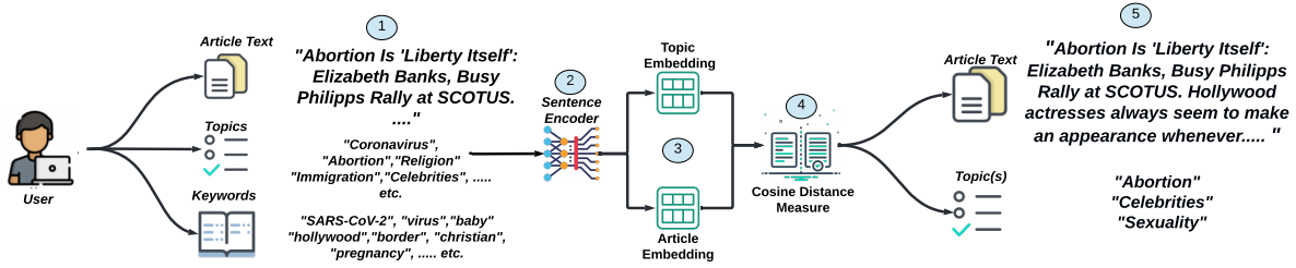
Figure 1: Steps for Zero-shot Multi-Label Topic Inference process, leveraging sentence encoders.
