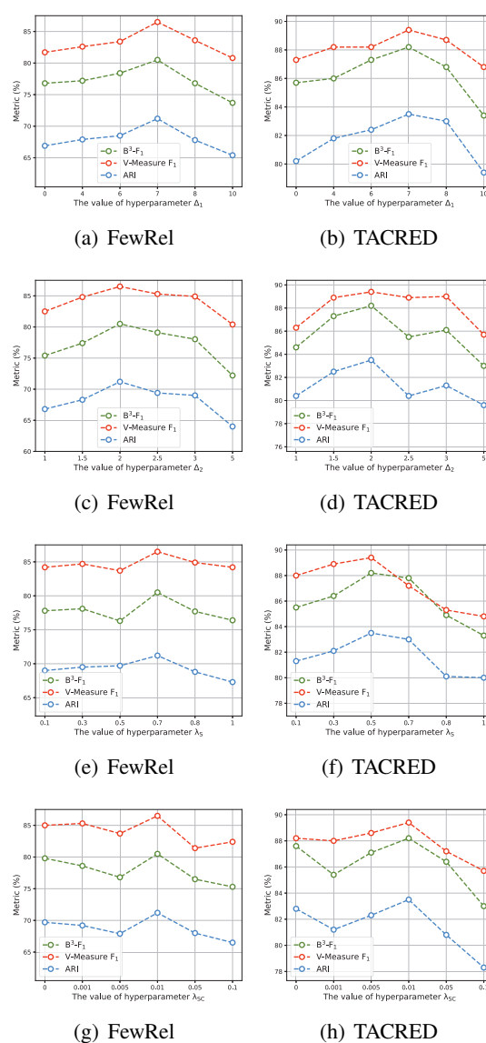
Figure 4: Hyperparameter Analysis.
