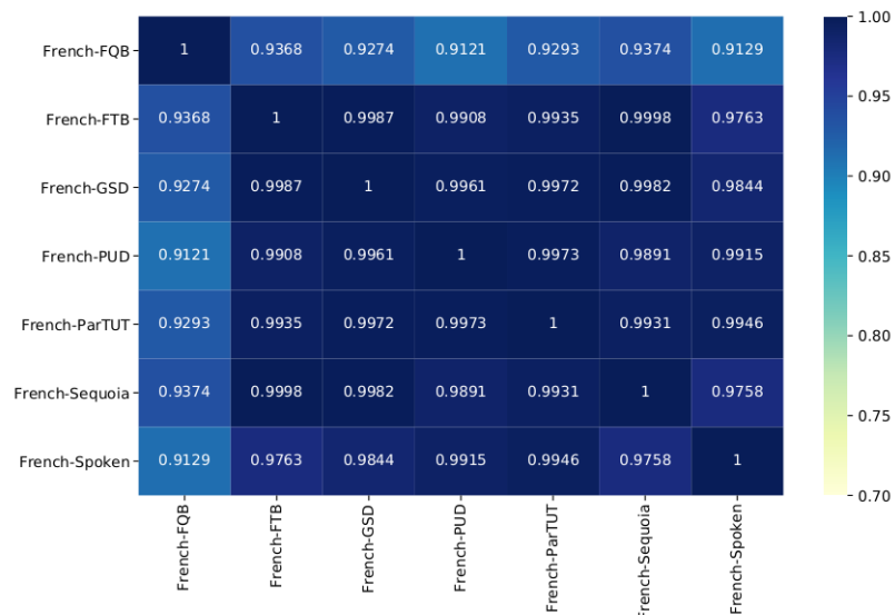
Figure 5: Cosine values between the seven French corpora in UD 2.7 1K .
