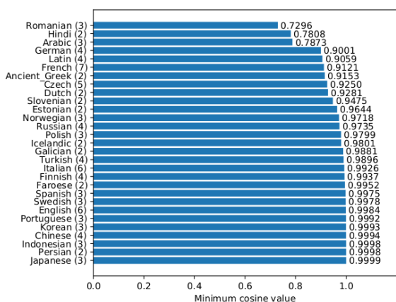
Figure 4: Multi-corpora (number in parenthesis) languages ordered by minimum cosine value.
