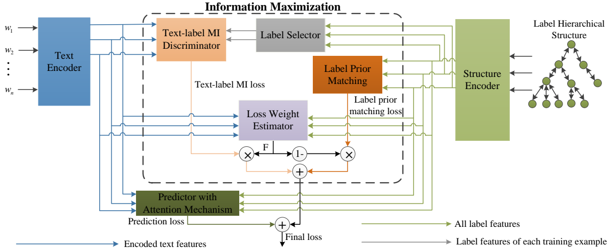
Figure 1: The architecture of our model HTCInfoMax.
