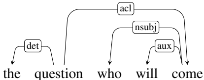
Figure 4: Enhanced graph of an interrogative clause.
