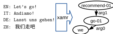
Figure 1: Cross-lingual AMR parsing as introduced by Damonte and Cohen (2018) .
