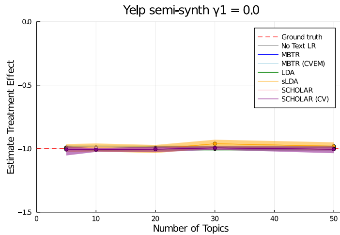
Figure 6: Without correlation between confounders and treatments, the regression can be dissected into two separate parts (supervised topic estimation and regression weight estimation of the non-text features) without inducing bias in the estimators, as described in the section on the Frisch-Waugh-Lovell theorem. In such a case, all models manage to recover the ground truth.
