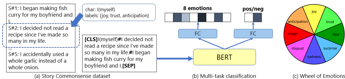
Figure 1: (a) Story Commonsense dataset, (b) emotion classification model, and (c) Plutchik’s Wheel of Emotions.
