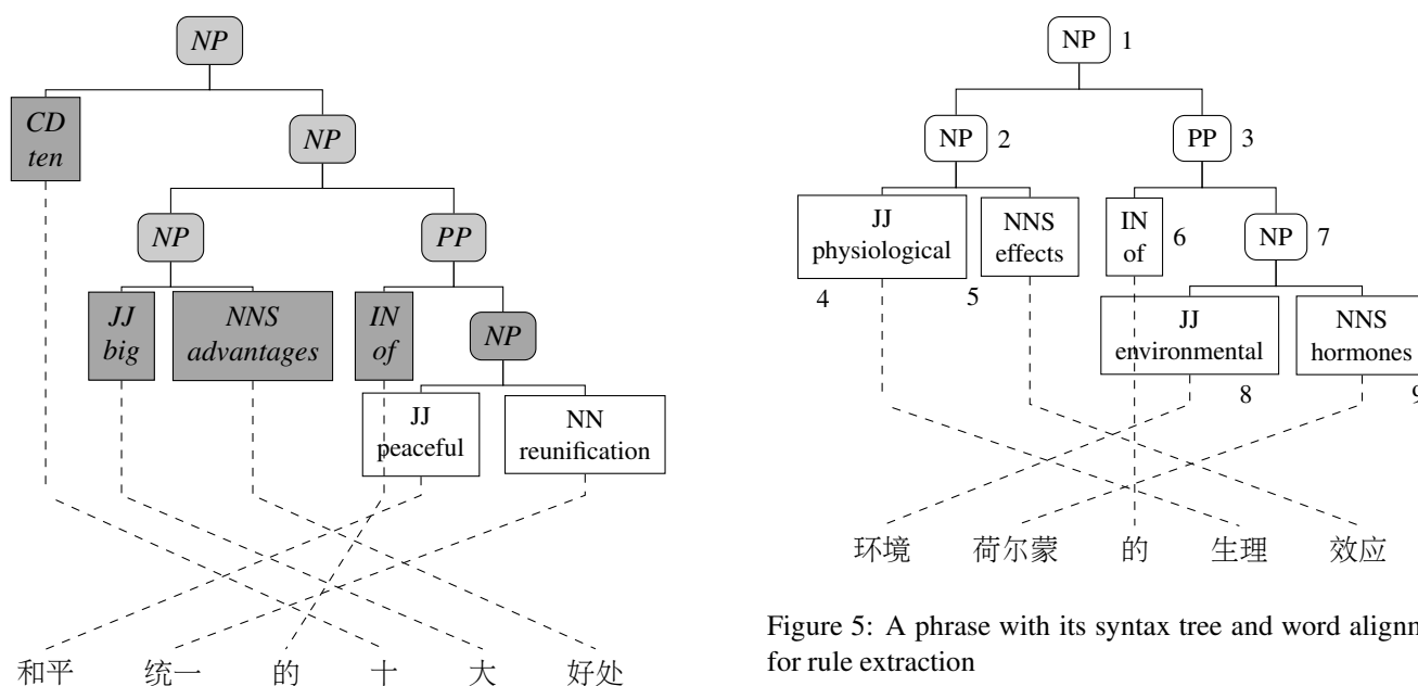
Figure 4: Detection of reordering pattern from multiple syntactic levels
