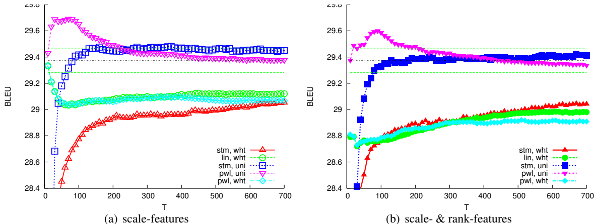
Figure 1: Comparison of weak learners, weighting schemes and feature sets on the WMT’10 test set. Weighting: uniform ( uni ), weighted with sentence-BLEU ( wht ). Learners: stumps ( stm ), linear ( lin ), piece-wise linear ( pwl ). Mean baseline MERT score is shown with 1\sigma interval.
