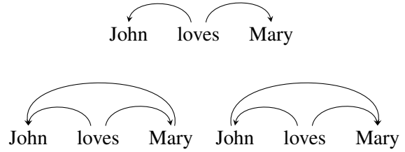
Figure 1: Possible spanning DAGs for John loves Mary .
