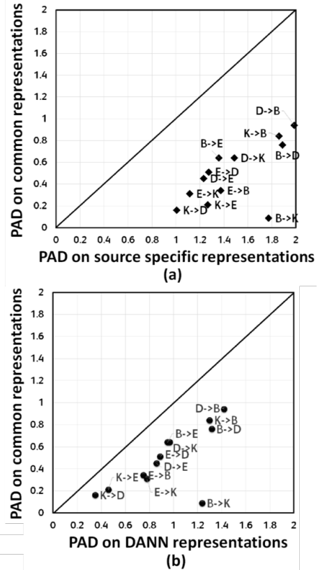
Figure 3: Compares the proxy – \mathcal{A} distances (PAD) computed on the common representations learned using the proposed technique v/s the (a) source specific and (b) representations learned using DANN.
