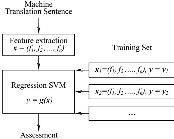
Figure 1: SVM based model of automatic MT evaluation metric
