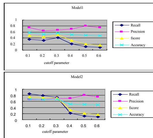
Figure 3. Test on human-annotated sentences
