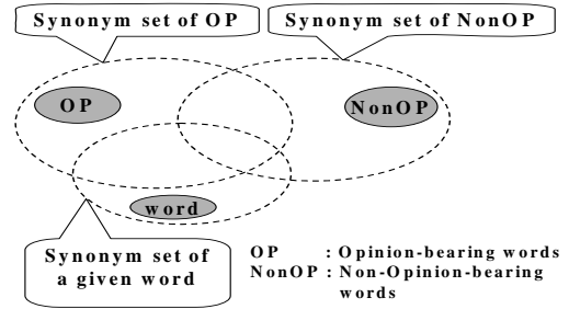
Figure 1. Automatic word expansion using WordNet
