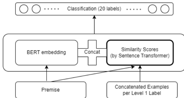
Figure 2: Hierarchical Similarity-aware model Architecture
