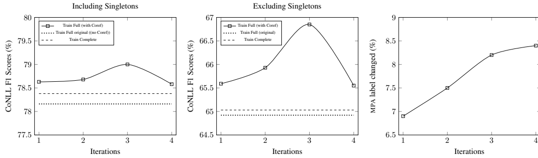
Figure 1: Left and Middle: The CoNLL scores for Yu et al. (2020) trained on different training sets and tested on the DEV set in gold mention setting. Right: The percentage of MPA labels changed by using the additional judgments from the Yu et al. (2020) system in different iterations.
