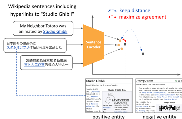
Figure 1: Illustration of the main concept behind EASE. Using a contrastive framework, sentences are embedded in the neighborhood of their hyperlink entity embeddings and kept apart from irrelevant entities. Here, we share the entity embeddings across languages for multilingual models to facilitate cross-lingual alignment of the representation.
