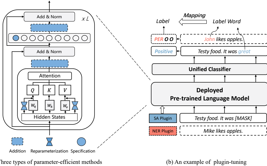
Figure 2: An overview of plugin-tuning. (a) is the three types of parameter-efficient methods, which can be used as our plugin. (b) shows the flow of plugin-tuning, we input the text and task-specific plugin to the deployed PLM, the PLM influenced by plugin outputs the label words in the sentence. The actual labels are obtained by label word mapping. “John” and “great” are label words selected by querying language model, respectively representing label “PER” for task NER and label “Positive” for task SA.
