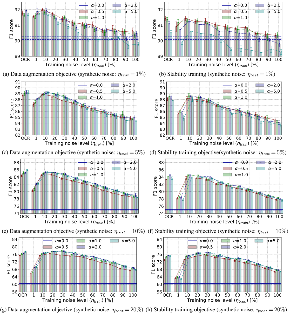
Figure 8: Extended results of our sensitivity analysis on the English CoNLL 2003 test data (§B.1). Each figure presents the results of models trained using one of our auxiliary training objectives on the original data perturbed with various levels of synthetic noise. The bar marked as "OCR" represents a model trained using the OCR noise distribution. Other bars correspond to models trained using synthetic noise distribution and different hyperparameters ( \alpha, \eta_{train} ).
