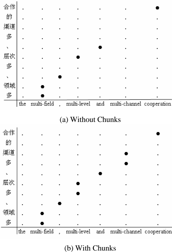
Figure 2. Alignment Examples w/o Chunks
