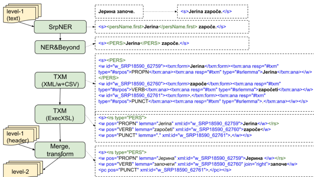
Figure 1: SrpELTeC level-2 pipeline illustrated by the sentence Јерина започе. (Jerina began.)
