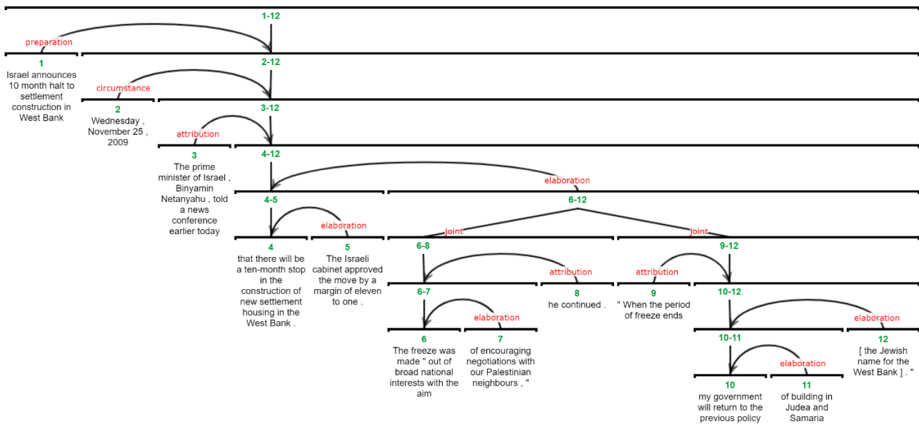
Figure 2: Predicted discourse parse for the same news text; errors compared to Figure 3 include viewing the circumstance clause ‘when the freeze ends’ as ATTRIBUTION and an incorrect attachment of the ELABORATION about the name of the West Bank. In contrast to the human analyst, the parser also groups units [6-12] as a JOINT, which is not implausible.
