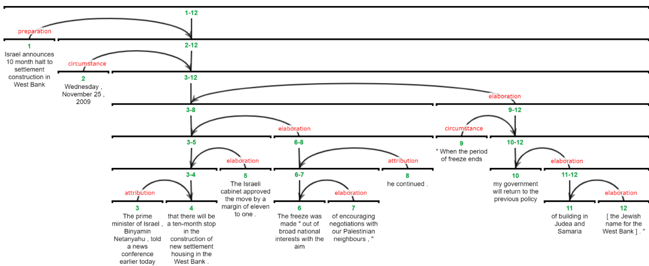
Figure 3: Manual discourse parse of the news text excerpt from Figure 2.
