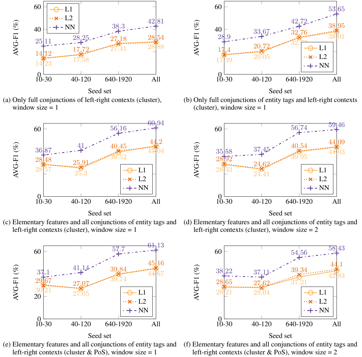
Figure 1: Average F1 of classification of unseen entity candidates on development data, with respect to the size of the seed. NN refers to models with nuclear norm regularization, L1 and L2 refer to \ell_1 and \ell_2 regularization. Each plot corresponds to a different conjunctive feature space with respect to window size (1 or 2), context representation (cluster with/out PoS), using entity features or not, and combining or not full conjunctions with lower-order conjunctions and elementary features.
