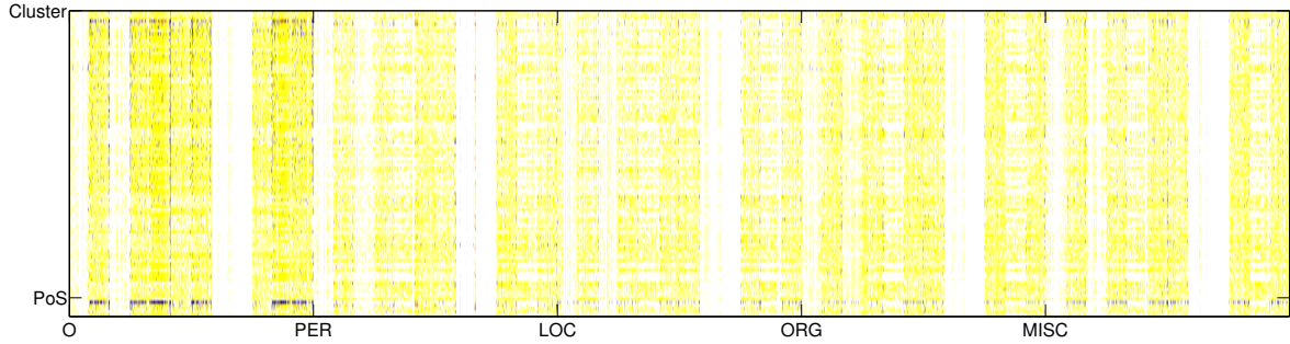
(a) Full parameter matrix of the low-rank model. The ticks in x-axis indicate the space for different entity types, while the ticks in y-axis indicate the space for different prefix context representations.
