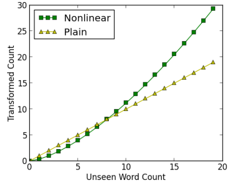
Figure 2: Nonlinear transformation of unseen word count with parameters set via cross-validation on the TREC training data: \alpha = 0.5 , \beta = 0 and \gamma = 1.5 .
