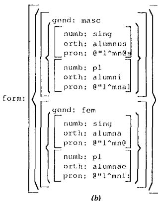
Fig. 13. Two different factorings of the same information
