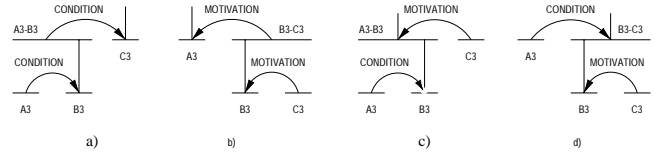
Figure 4: The set of all RS-trees that can be built for text (11).
