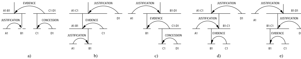
Figure 1: The set of all RS-trees that can be built for text (1).
